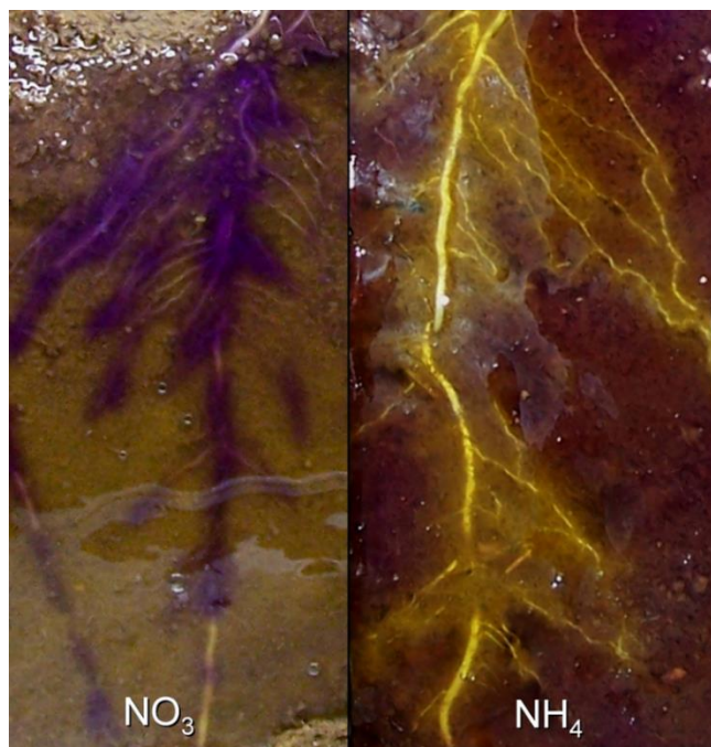
Fig. 2. Bromocresol purple, a pH indicator, added to soil turns purple at high pH in association with uptake of nitrate. Or it turns yellow at low pH with the uptake of N as ammonium.
