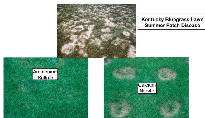
Fig. 3. Ammonium nutrition suppresses summer patch disease on Kentucky bluegrass.
